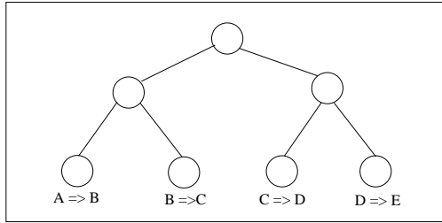
Figure 7: A decomposition tree for the theory A \supset B, B \supset C, C \supset D, D \supset E .
